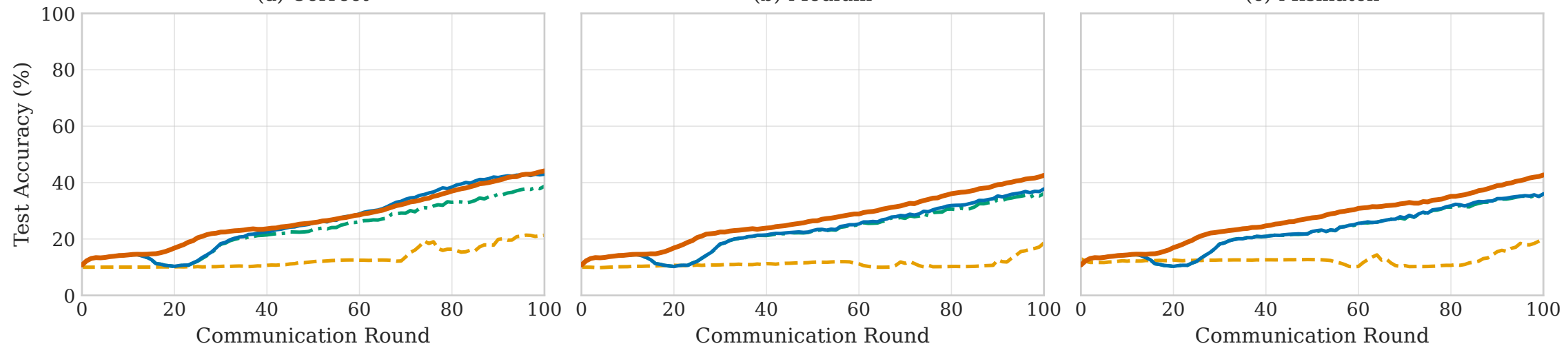
(a) Correct
