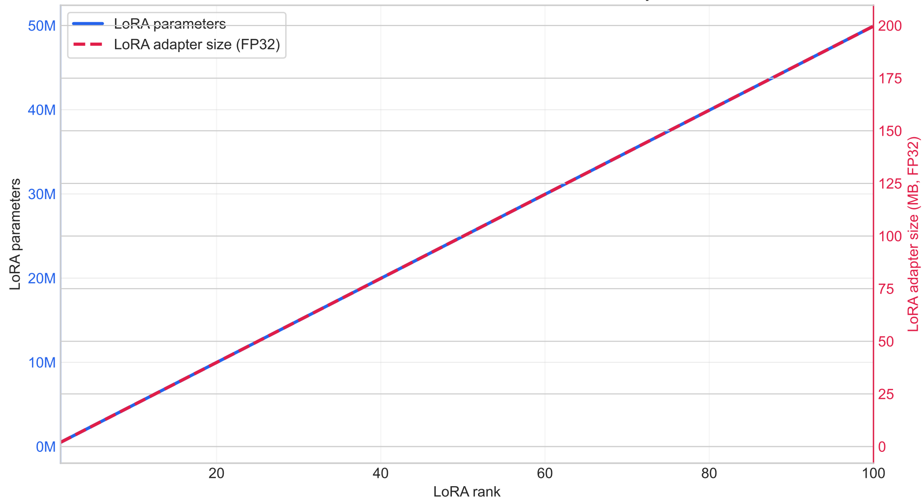
RoBERTa: LoRA Rank vs. Parameter Count and Adapter Size
