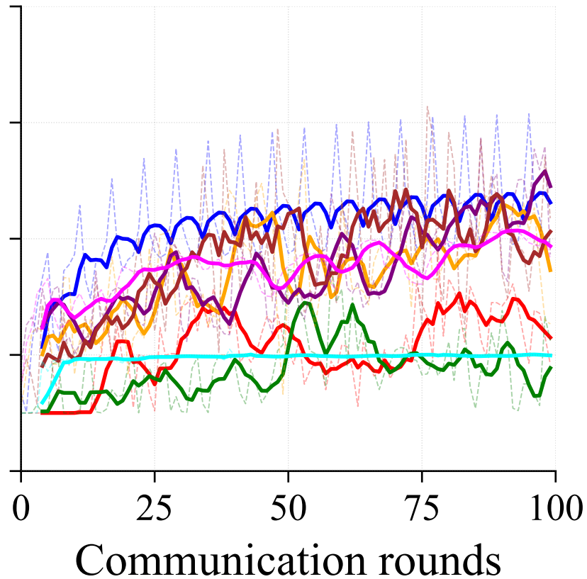
AWS FMNIST
