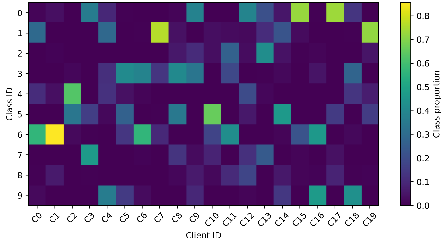
Client-Class Distribution under Non-IID Setting
