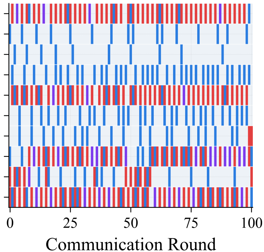
FMNIST
