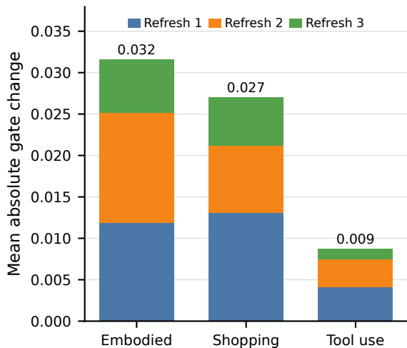
(c) Plasticity budgets
