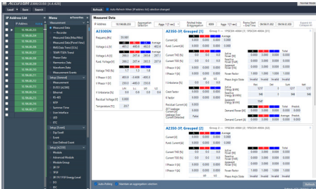
Measurement Data Collection Interface
