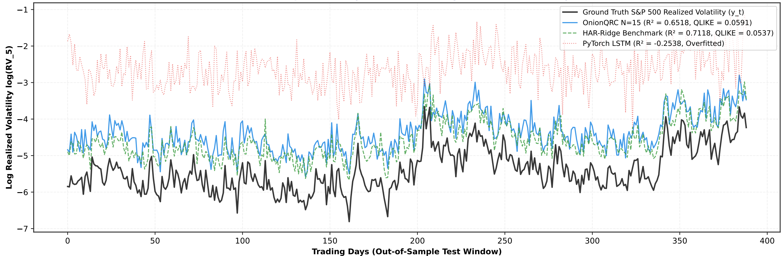
Out-of-Sample Volatility Forecast Tracking (Test Set N=389 Days)
