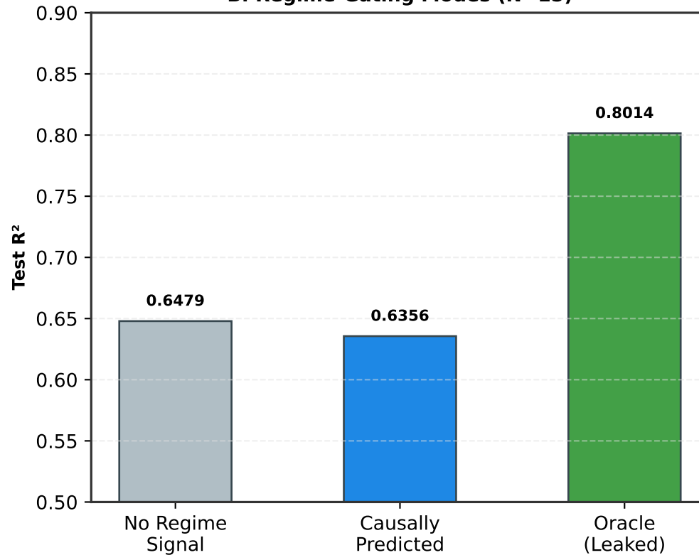
B. Regime-Gating Modes (N=15)
