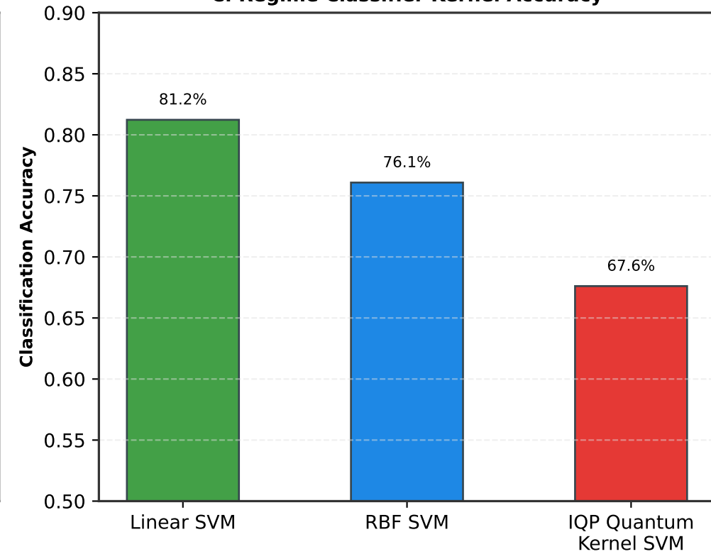
C. Regime Classifier Kernel Accuracy
