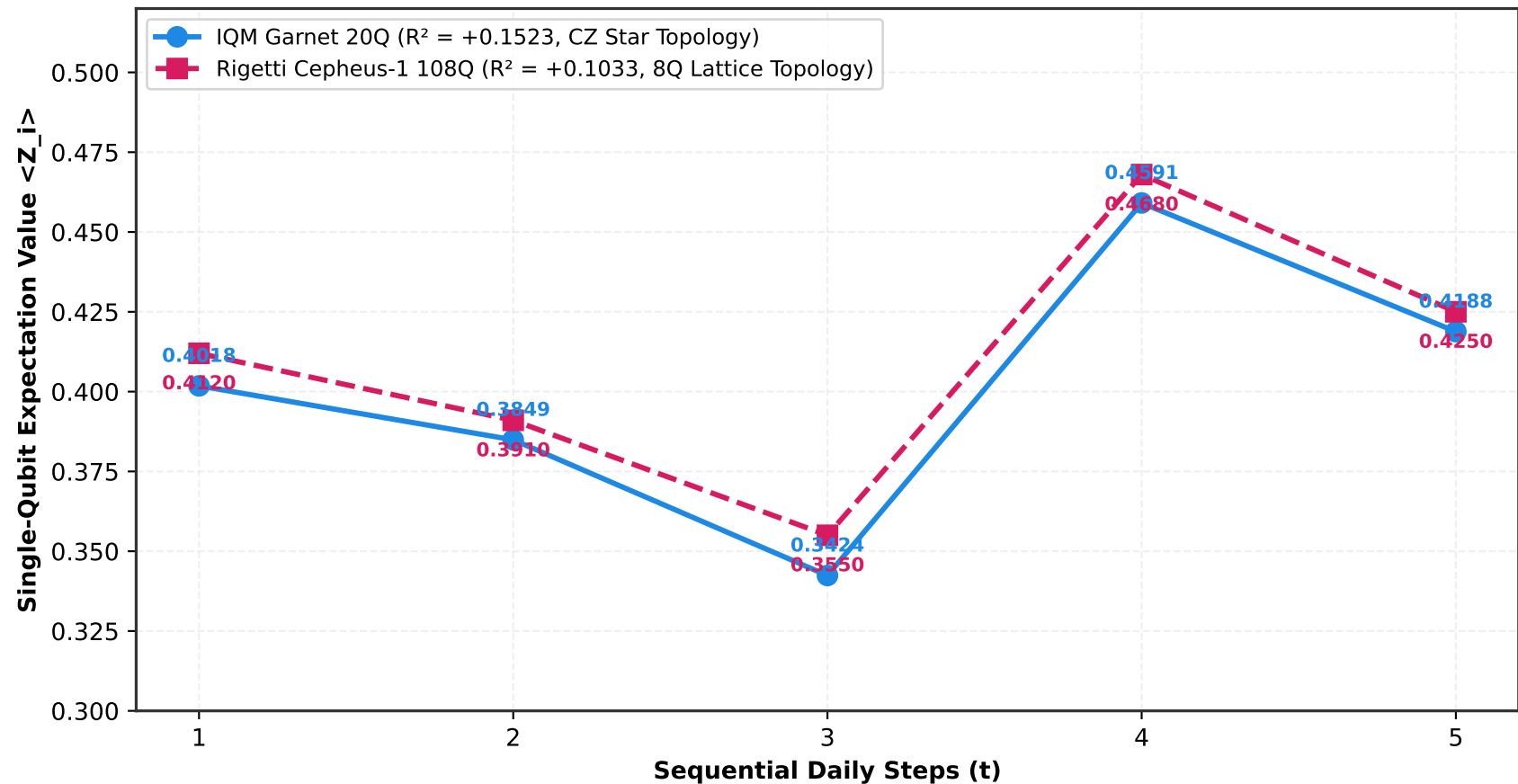
Physical Recurrent QPU Memory Dynamics Across 5 Sequential Trading Days
