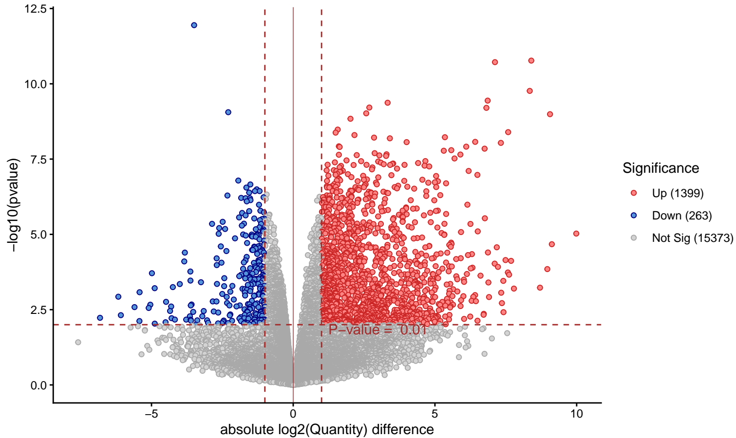
Volcano plot
