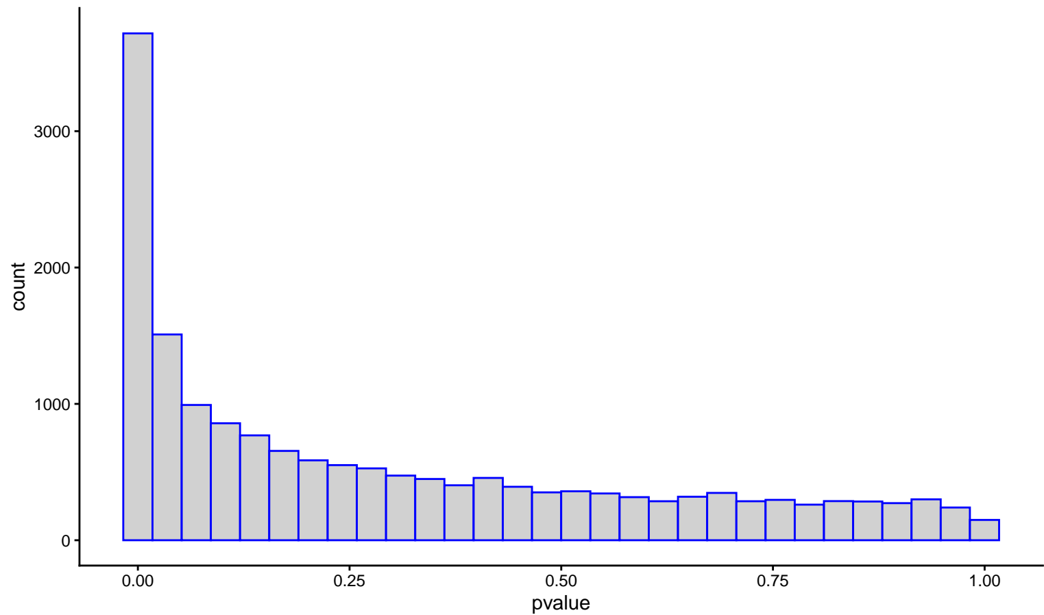
P value histogram
