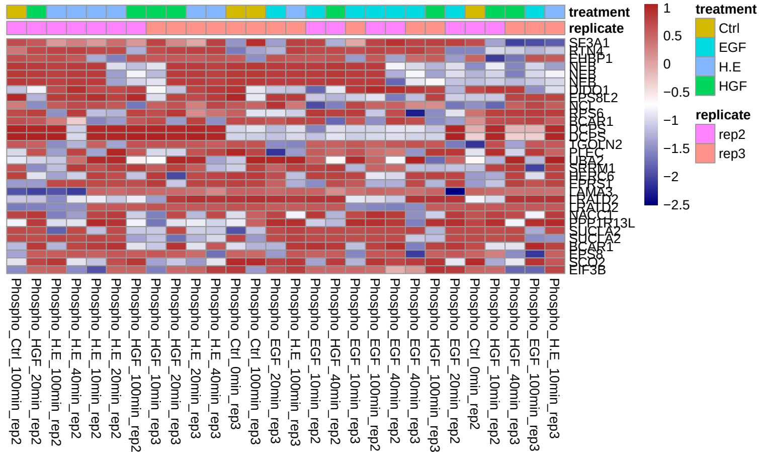
Top variant
