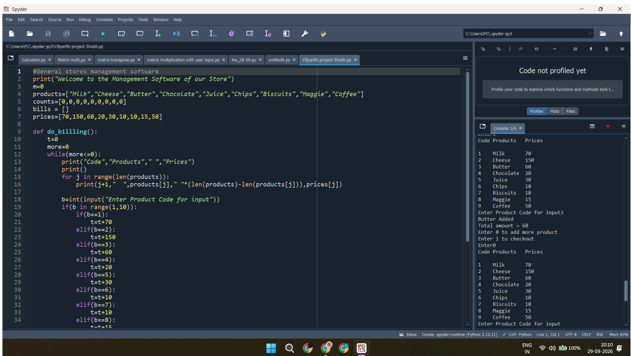
Figure 4. Product selection and billing output.
