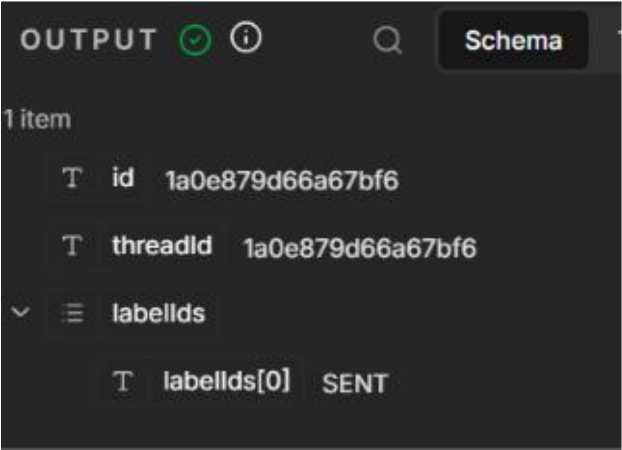
Figure 10. Processing Notification
