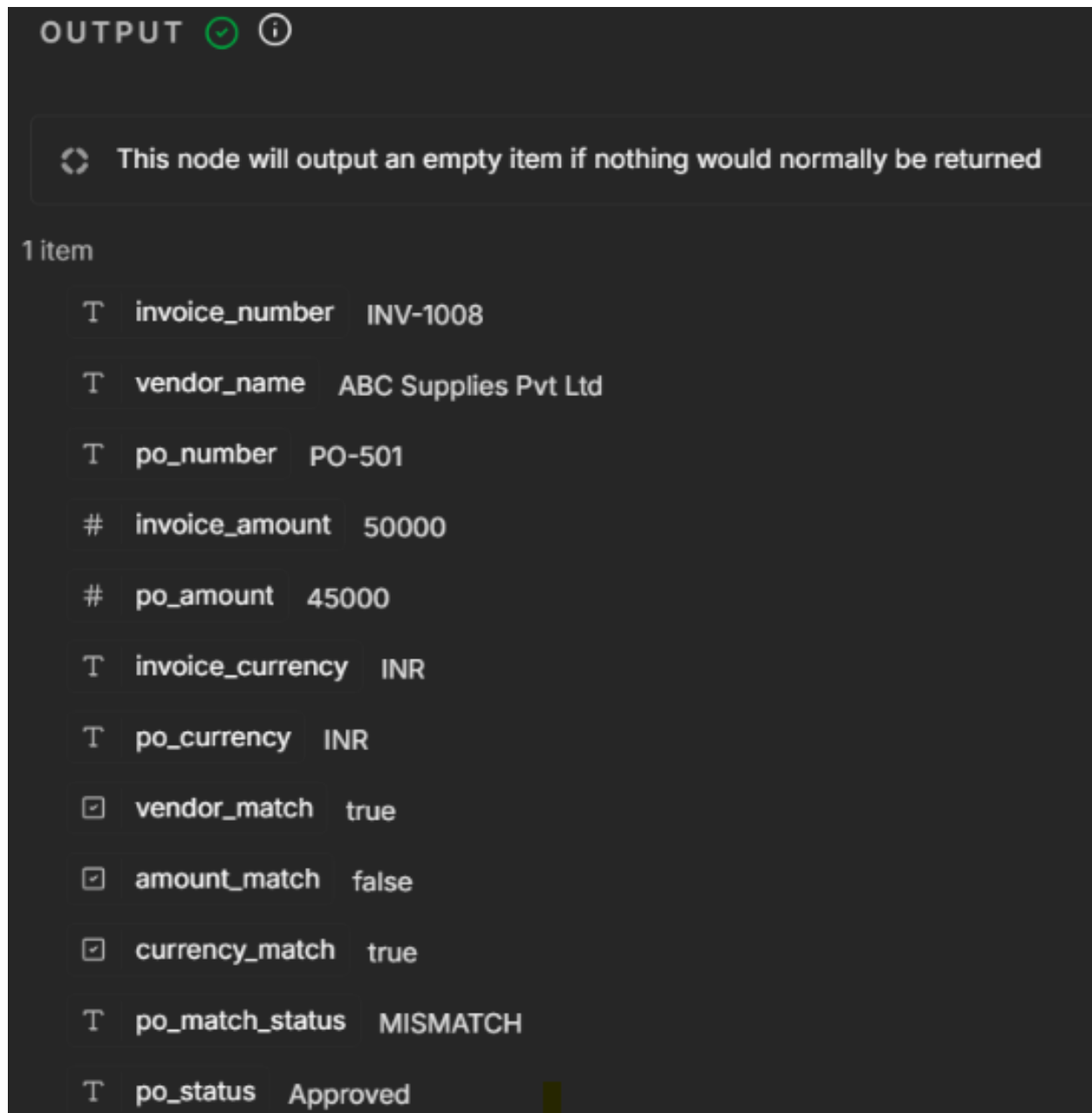
Figure 6. PO & Vendor Validation
