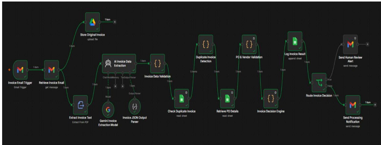
Figure 1. Final n8n Workflow
