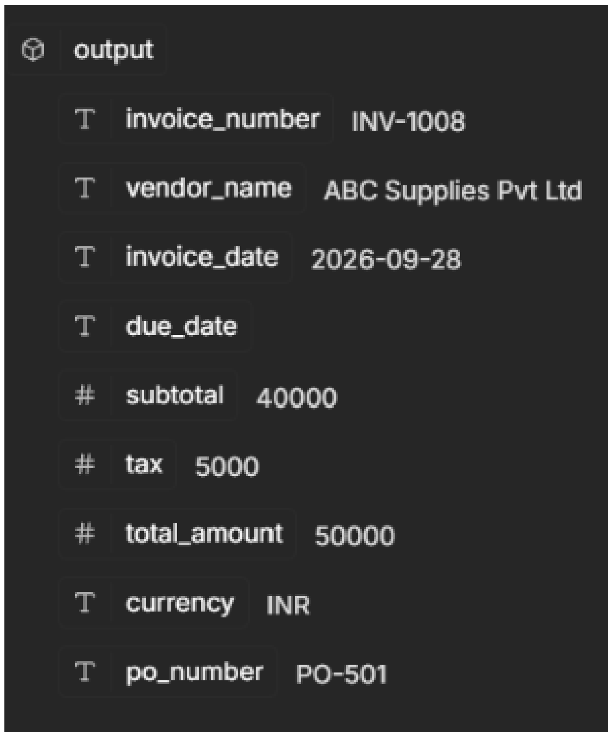
Figure 3. Gemini Invoice Extraction
