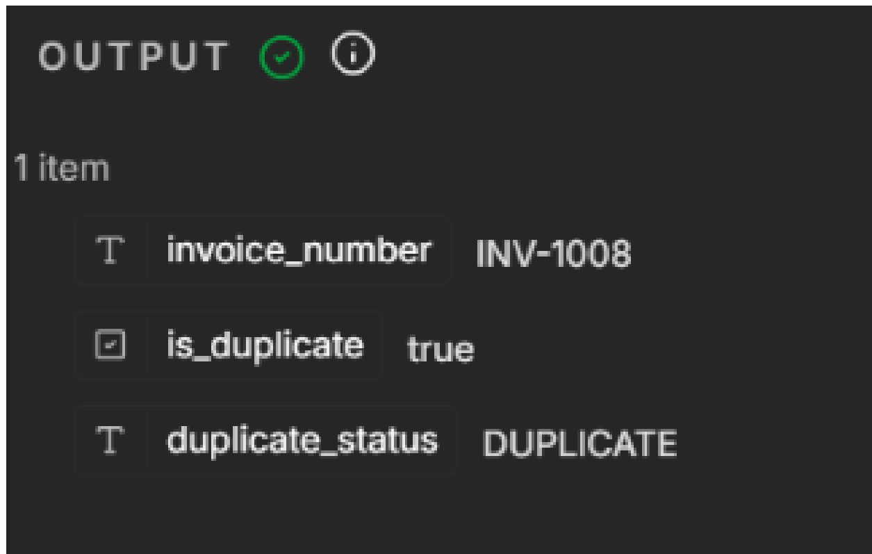
Figure 5. Duplicate Detection
