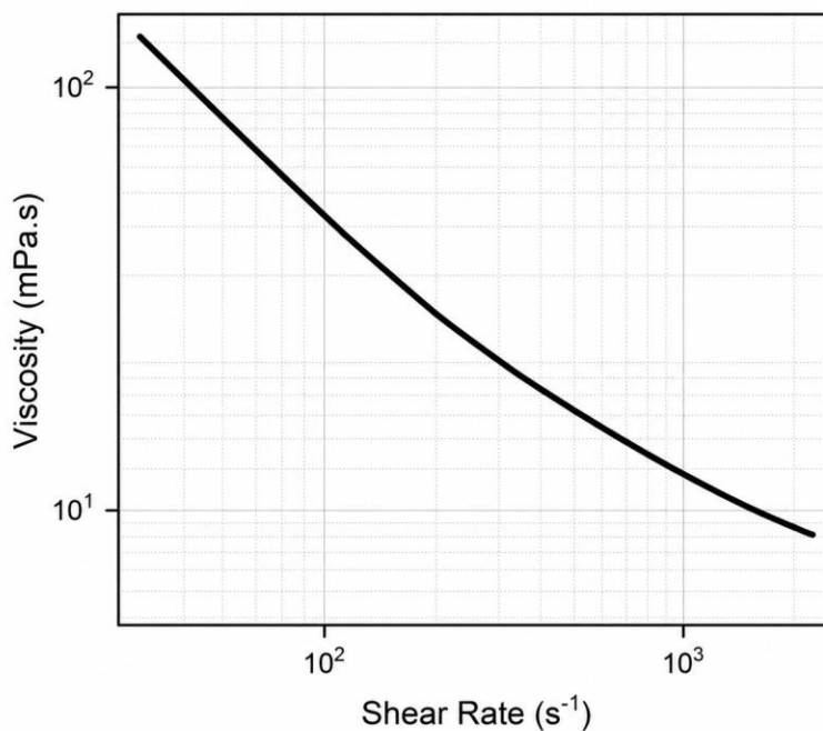
Rheology Curve
