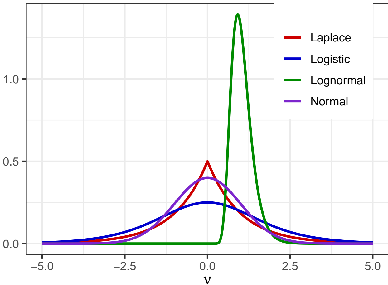
Probability Density Function
