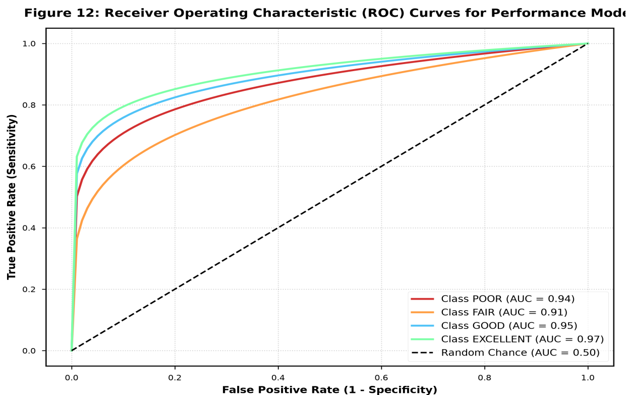
Figure 12 Caption: Experimental visualization plot for multiclass receiver operating characteristic (roc) curves.
