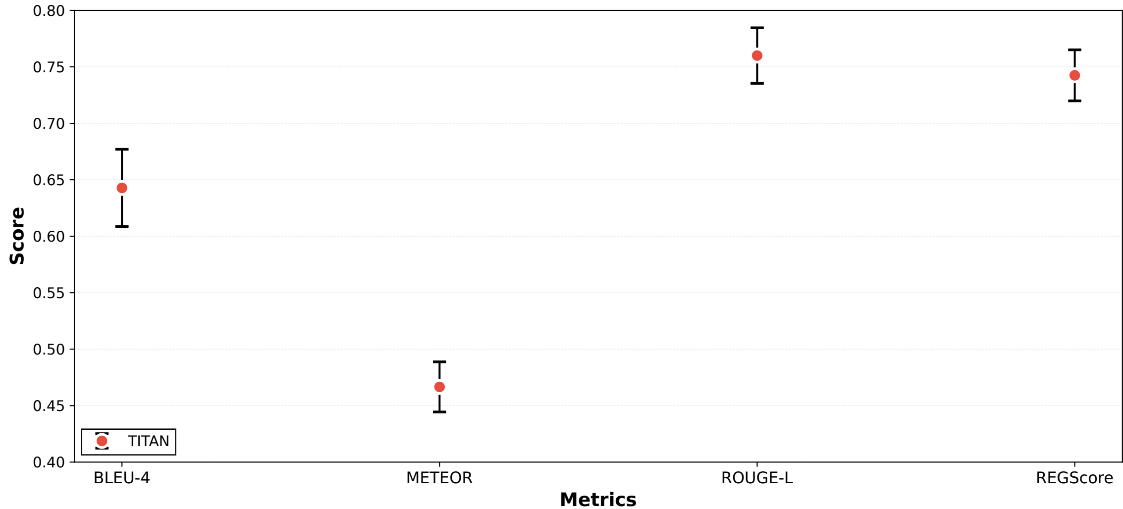
TITAN Performance Across Metrics
