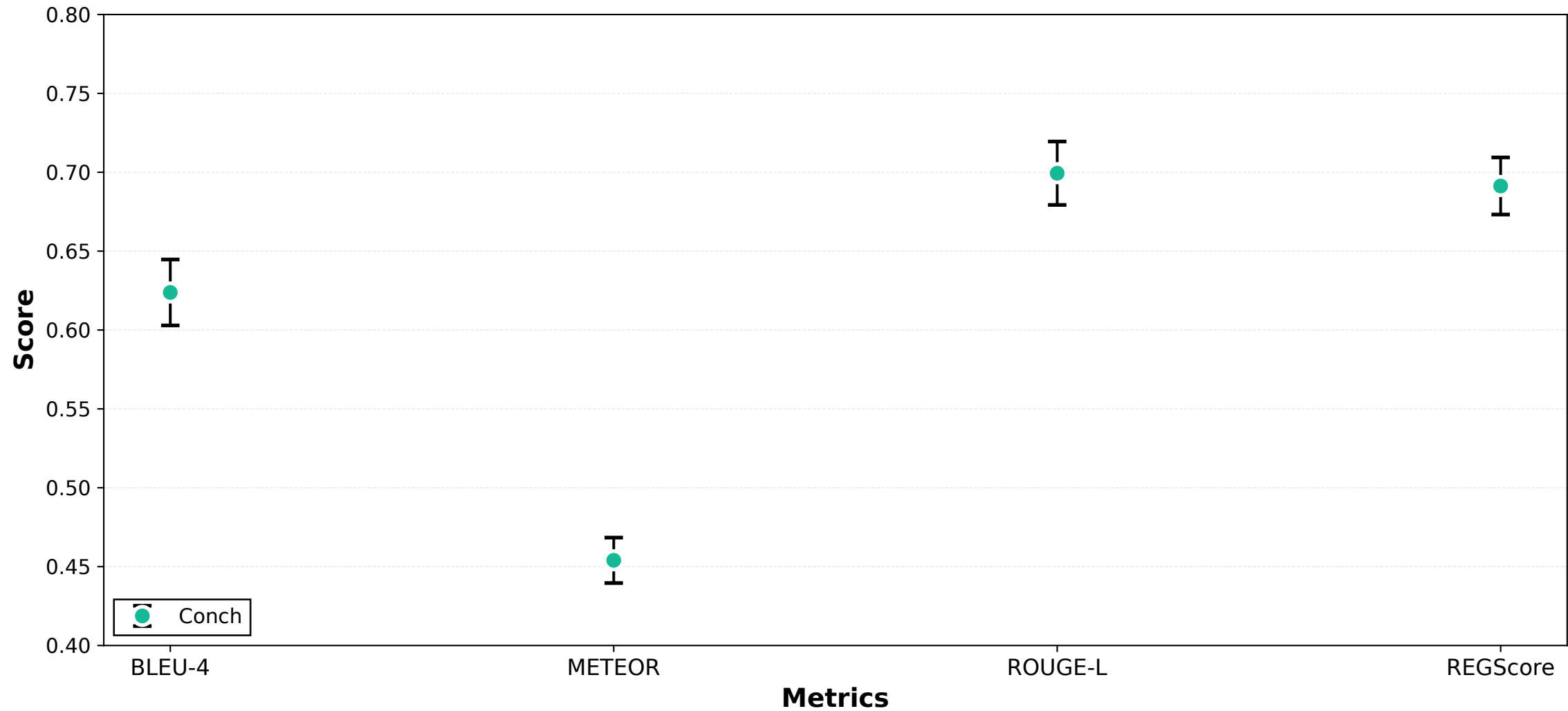
Conch Performance Across Metrics
