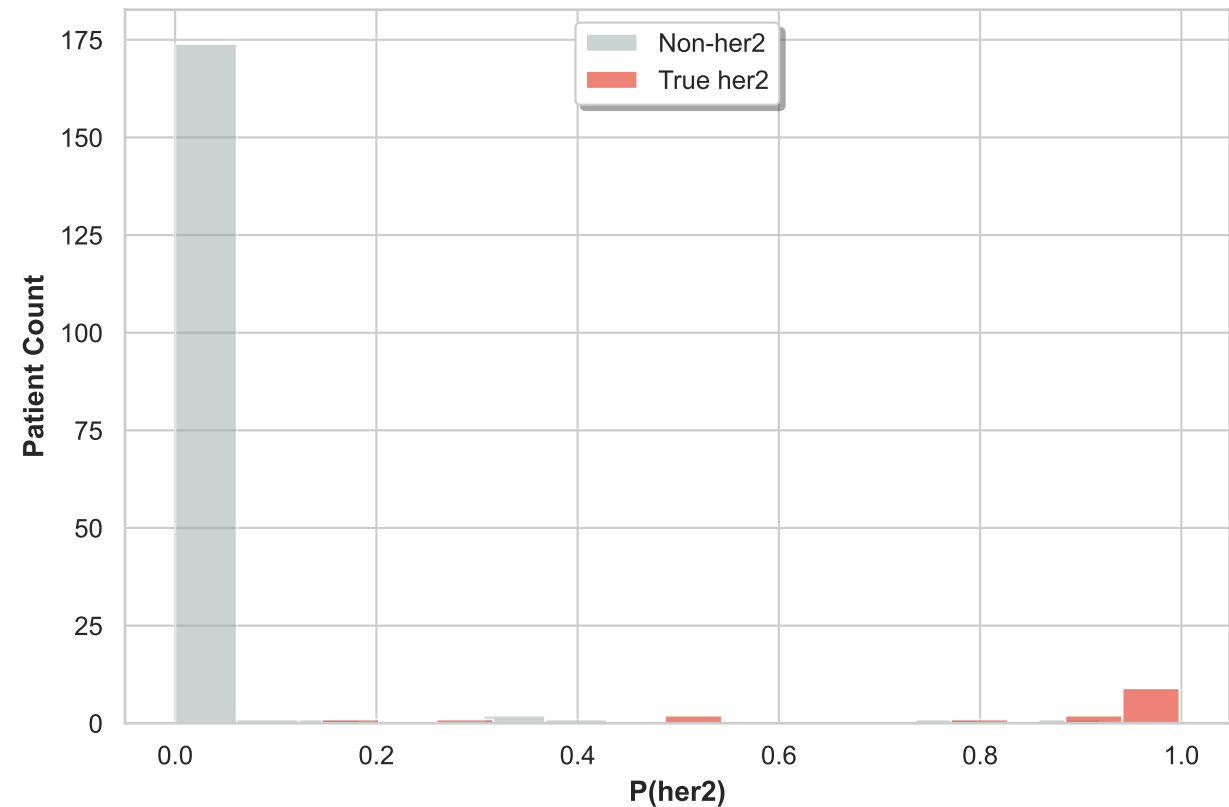
Probability Distribution: HER2
