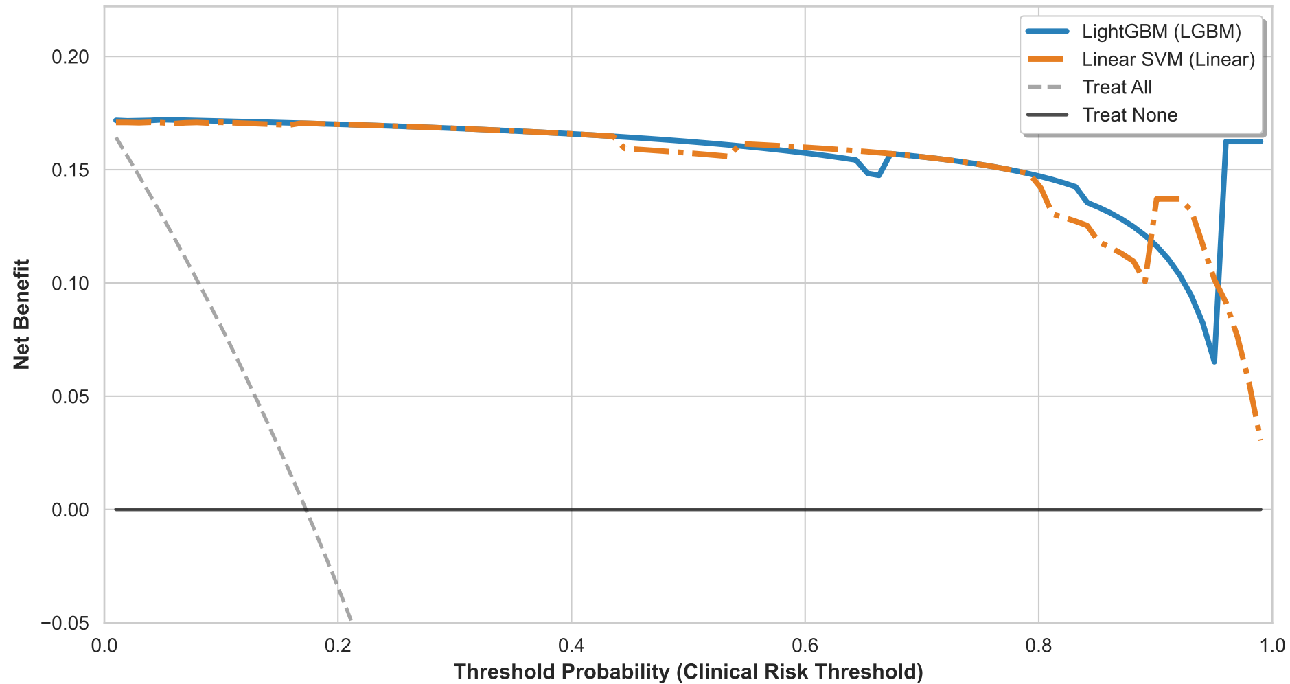
Clinical Decision Curve Analysis (DCA) Target: Basal (TNBC) Subtype
