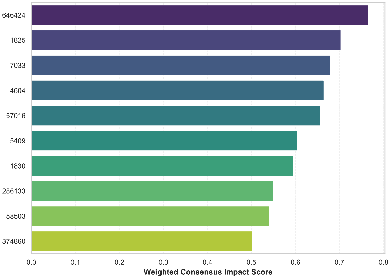
Subtype: LUMINAL_A Consensus Feature Importance
