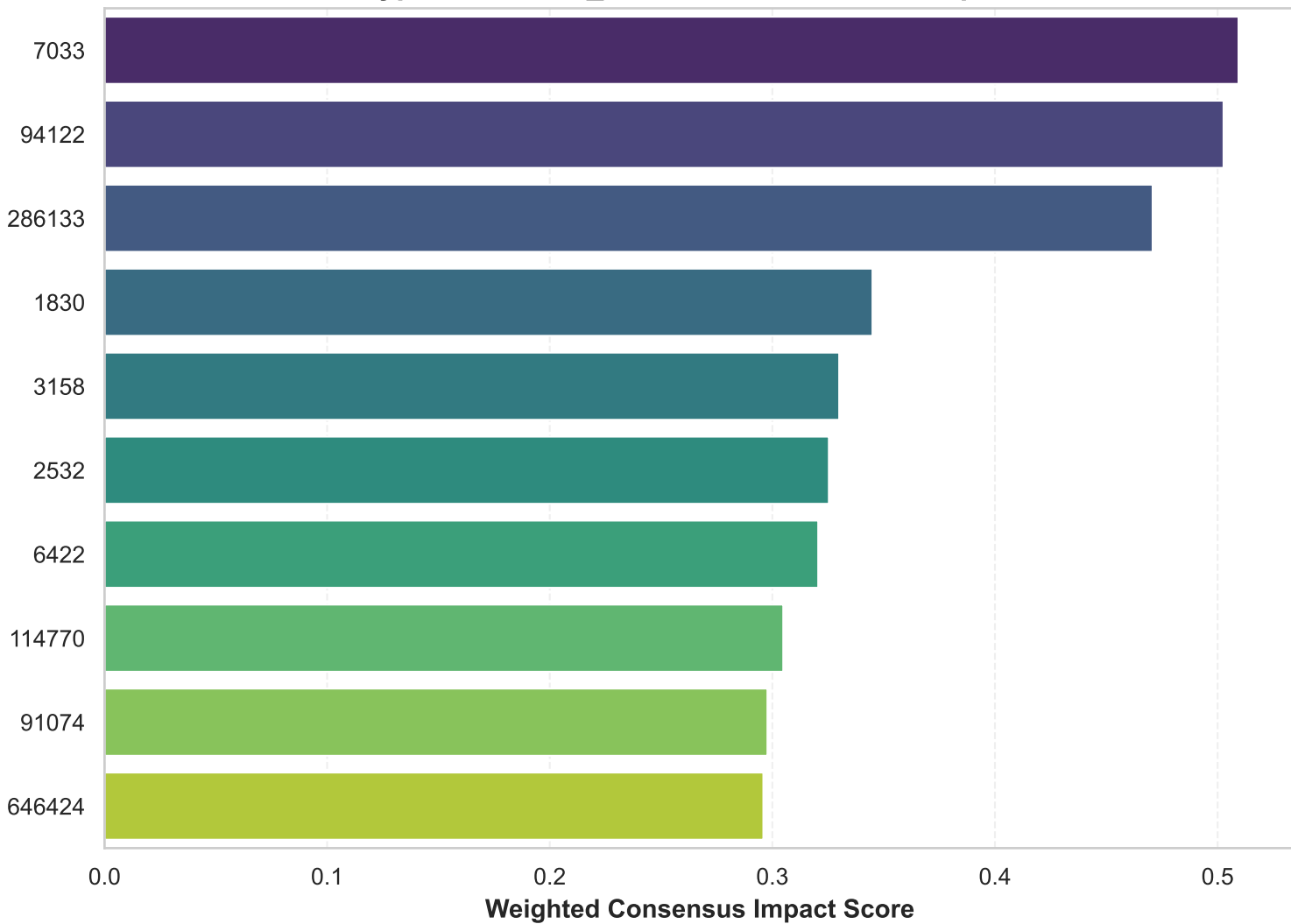
Subtype: LUMINAL_B Consensus Feature Importance
