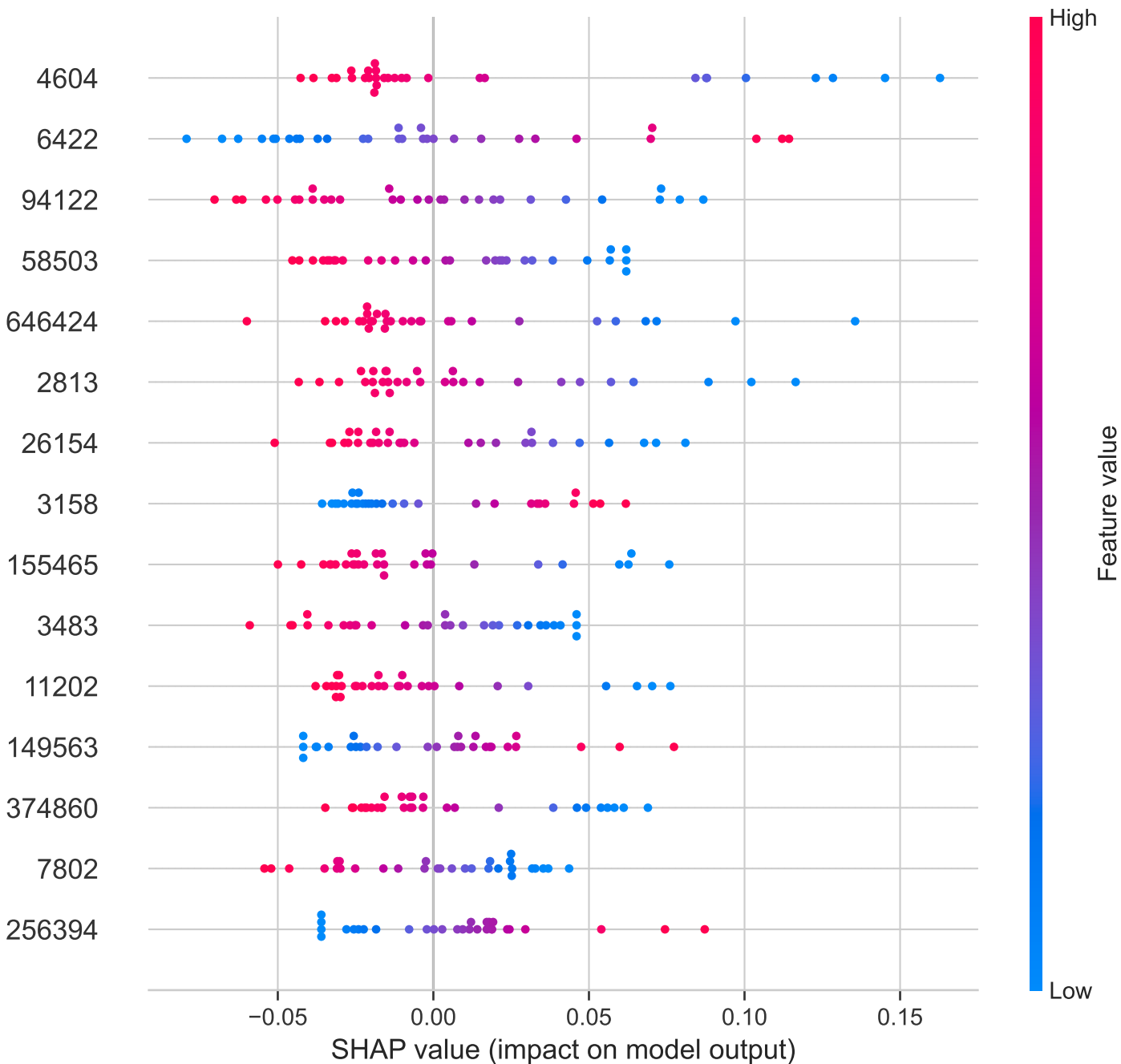
Standard SHAP Summary Beeswarm Plot: Linear SVM
