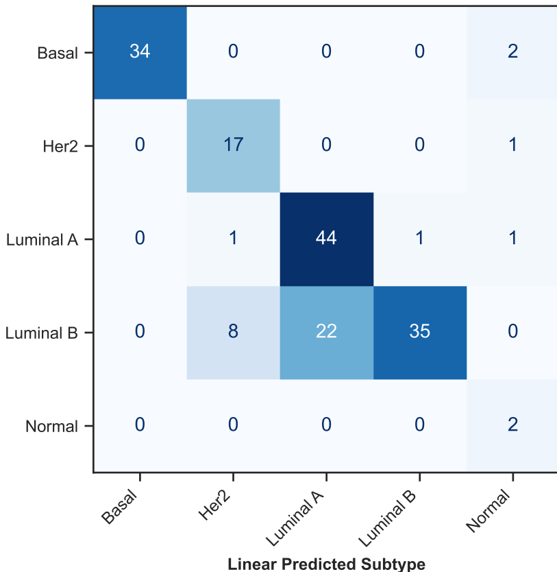
Confusion Matrix: SMC 2018 (Linear SVM Transfer) Macro F1: 0.743
