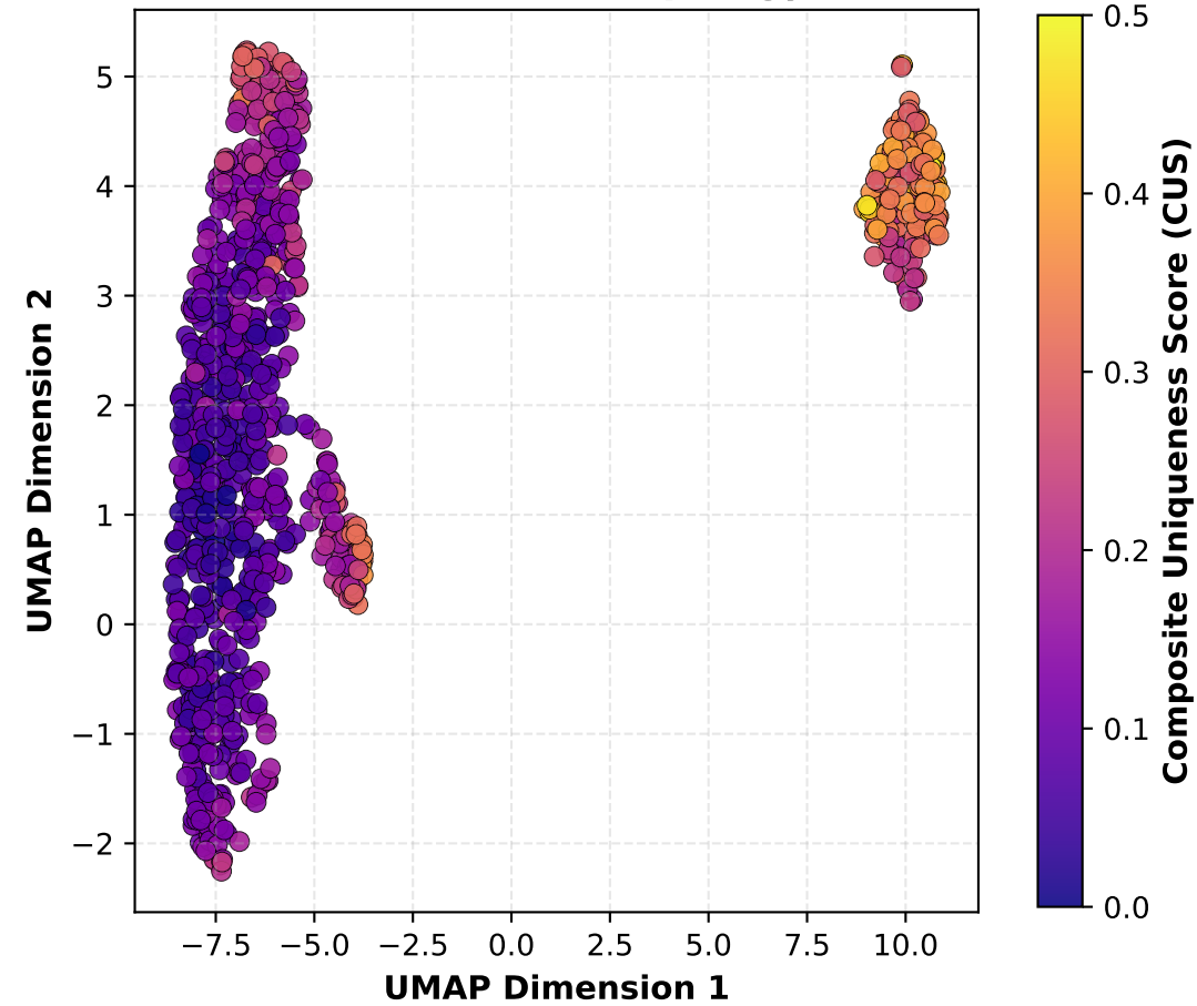
UMAP: Latent Topology
