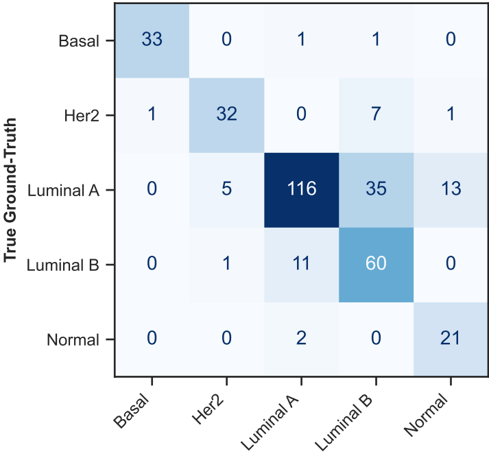
Linear Predicted Subtype SCAN-B | SVM Transfer Macro F1: 0.792
