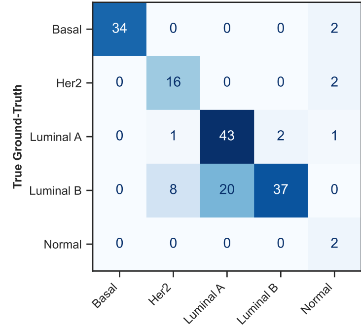
Linear Predicted Subtype SMC 2018 | SVM Transfer Macro F1: 0.695
