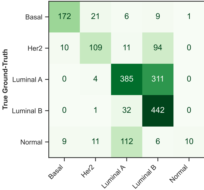
Linear Predicted Subtype METABRIC | SVM Transfer Macro F1: 0.571
