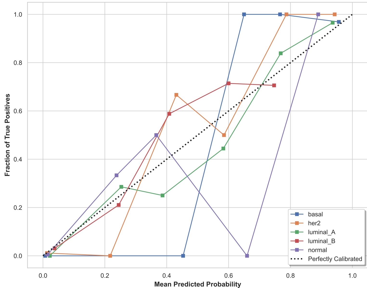
Support Vector Machine (RBF) Proof of Probabilistic Reliability
