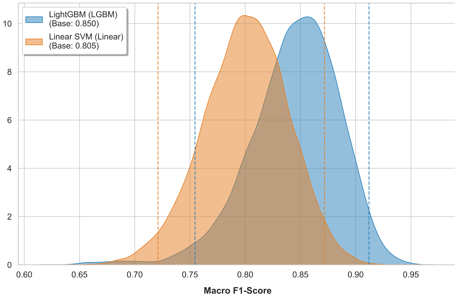
Bootstrap Distribution of Holdout Macro F1-Score (N=10,000)
