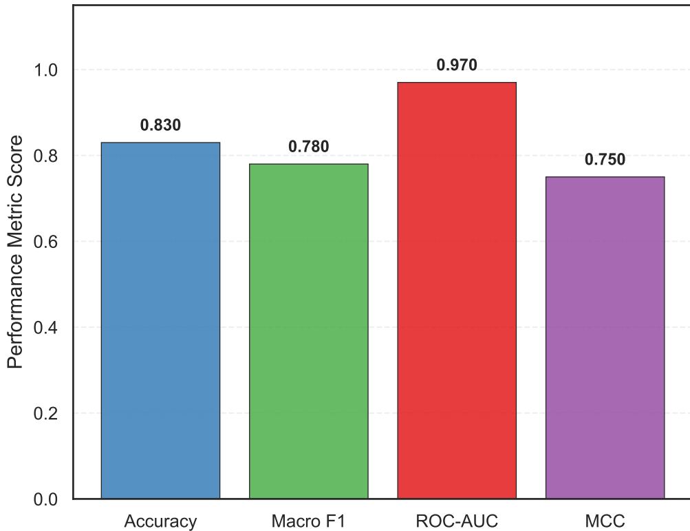
External Validation Performance - SCAN-B
