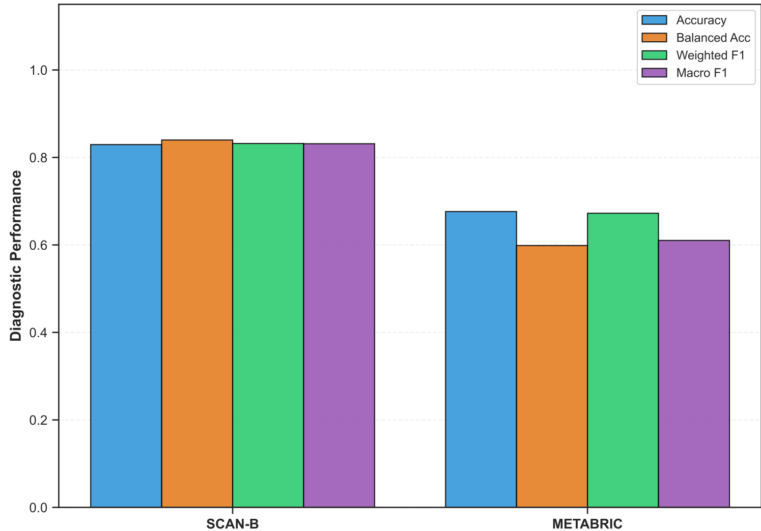
Cross-Platform Validation: Linear Model (Linear SVM)
