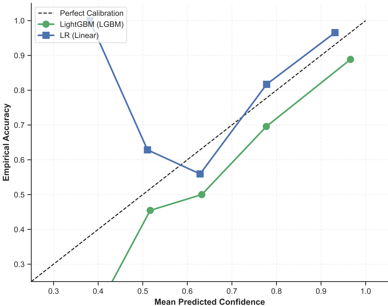
Clinical Probability Calibration Diagram Cohort: SCAN-B
