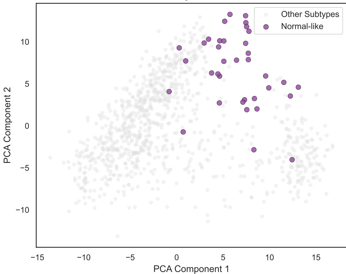
PCA Manifold Projection - Normal-like
