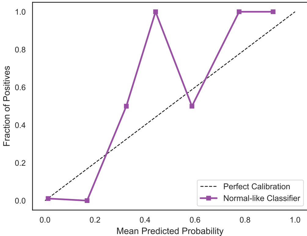
Clinical Reliability Diagram - Normal-like
