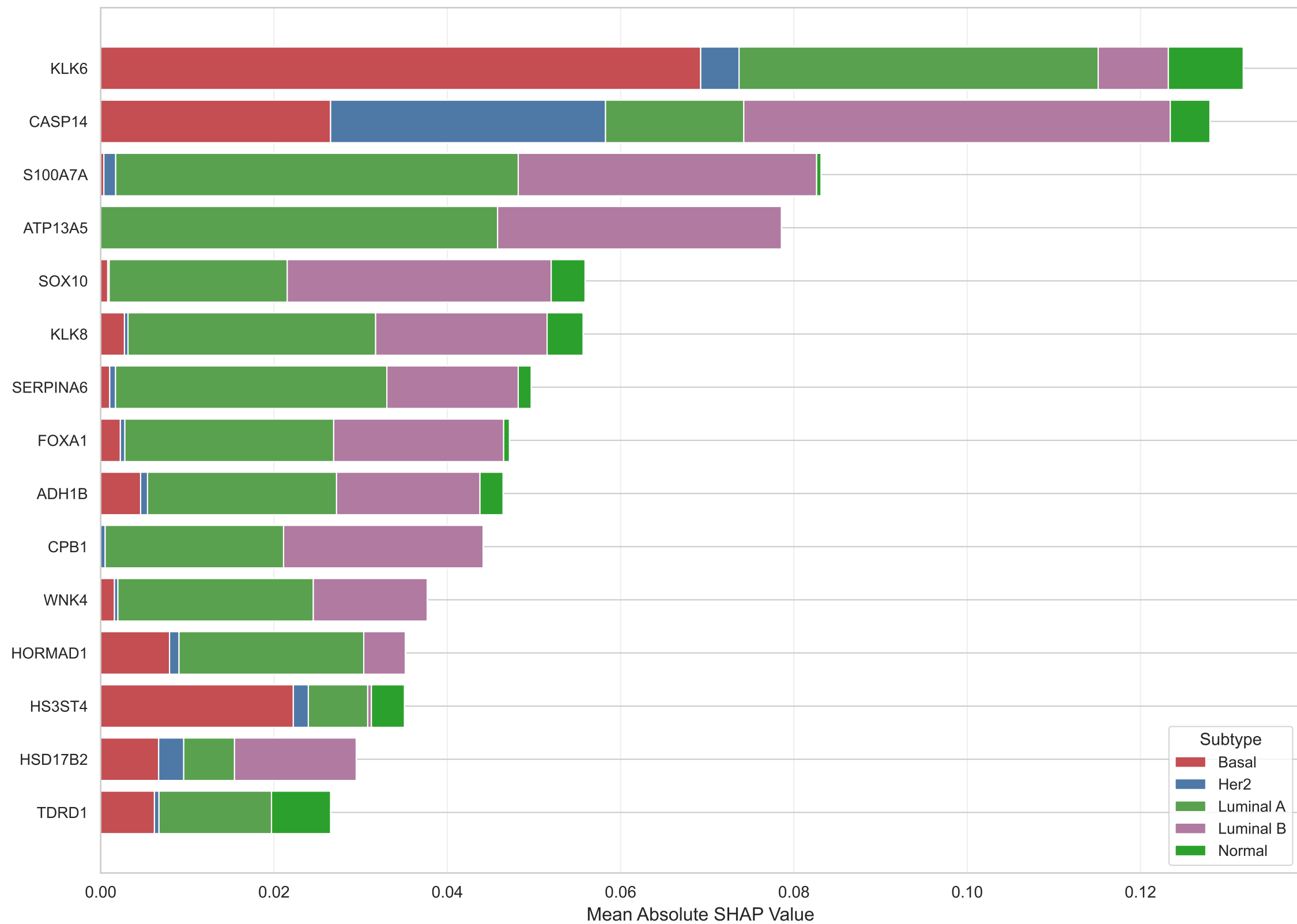
Multi-Class SHAP Impact: LightGBM (LGBM)
