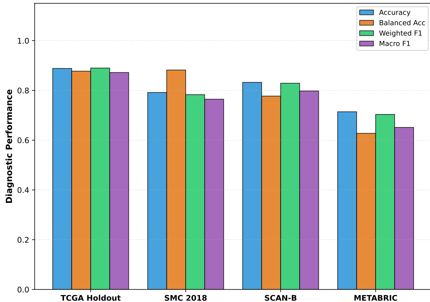
Cross-Platform Validation: Non-Linear Model (RBF-SVM)
