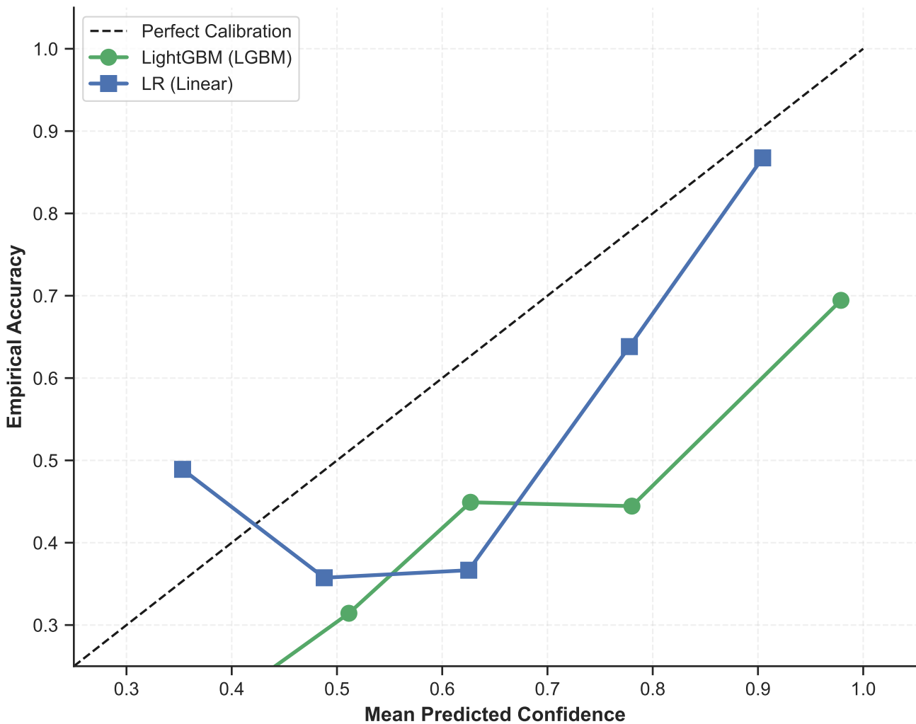
Clinical Probability Calibration Diagram Cohort: METABRIC
