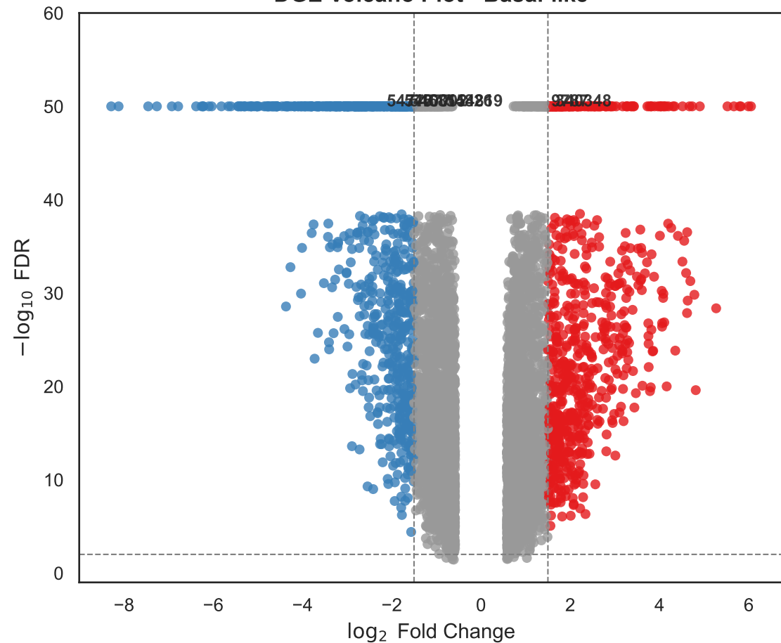
DGE Volcano Plot - Basal-like
