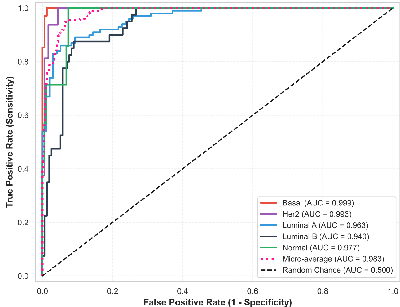
Overall Multi-Class ROC Curves (Unseen Holdout Cohort, N=197)
