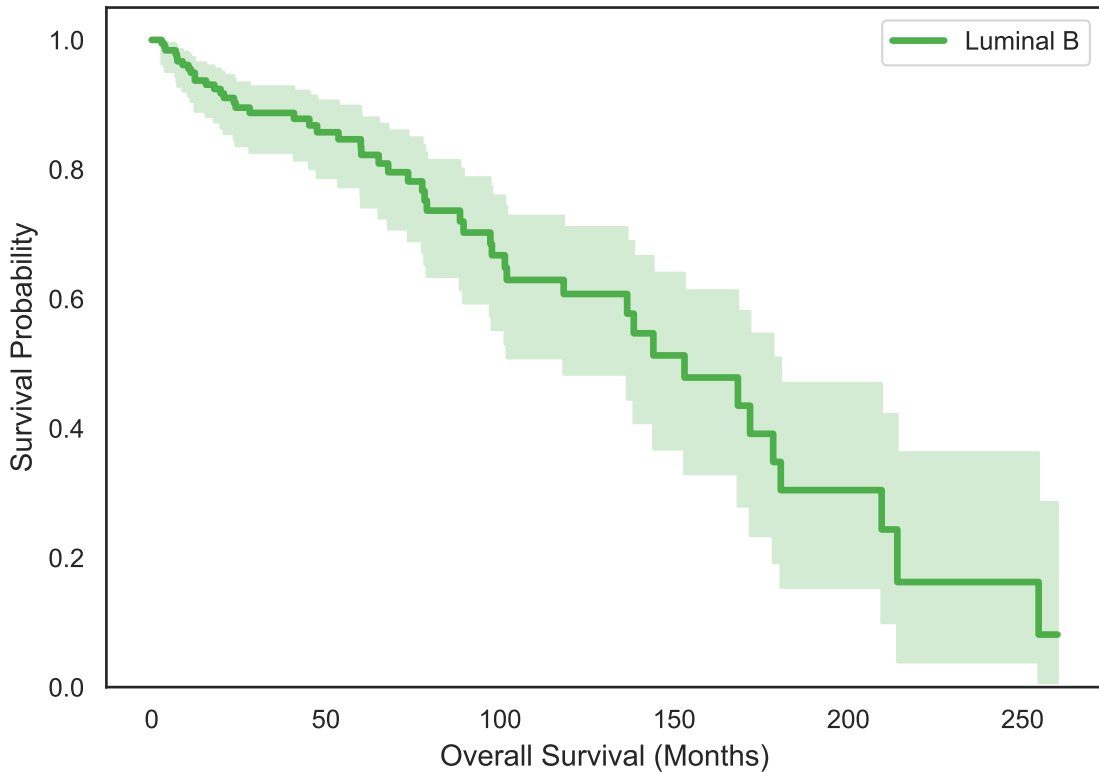
Kaplan-Meier Survival Curve - Luminal B
