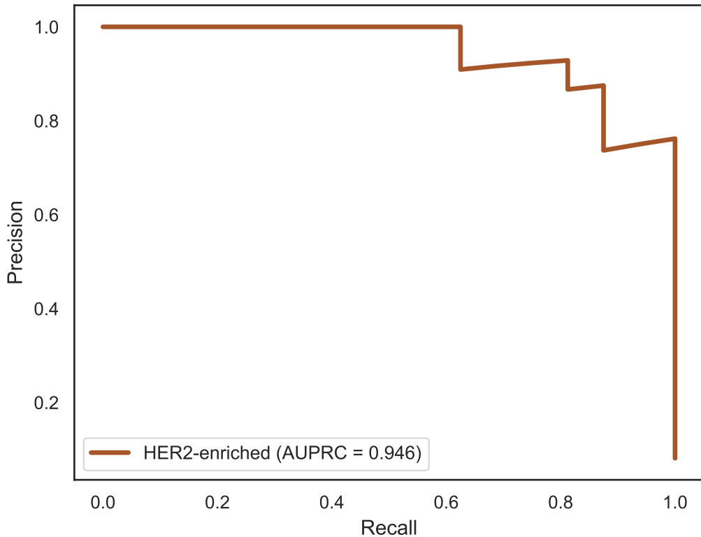
Precision-Recall Curve - HER2-enriched
