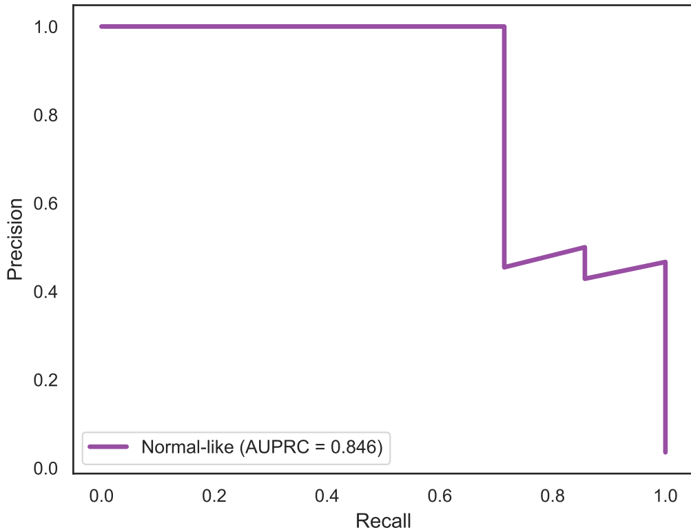
Precision-Recall Curve - Normal-like
