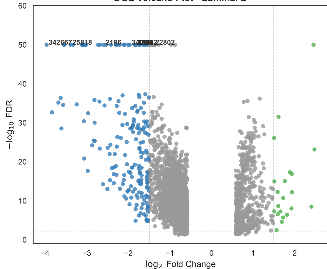
DGE Volcano Plot - Luminal B
