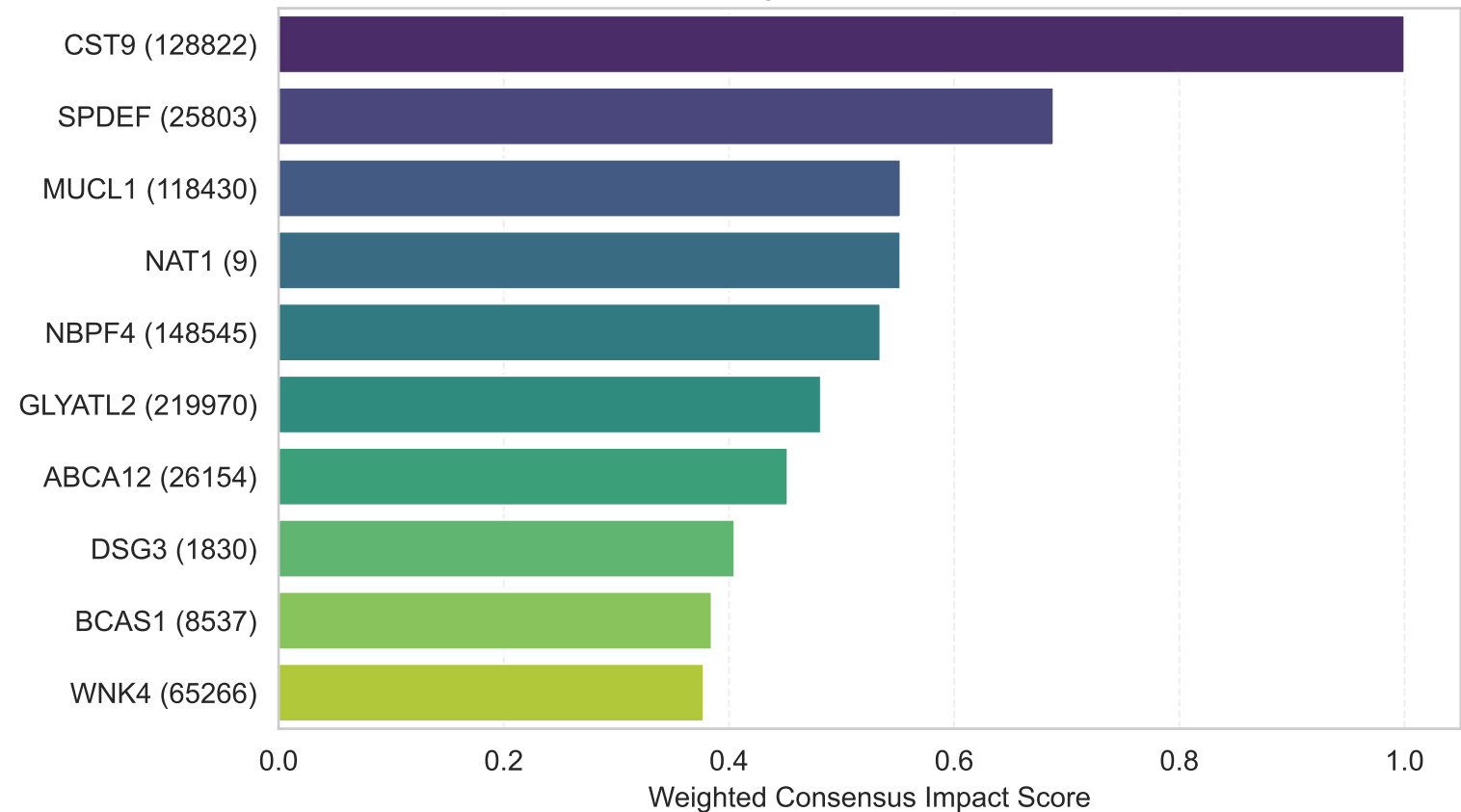
Subtype: LUMINAL_A
