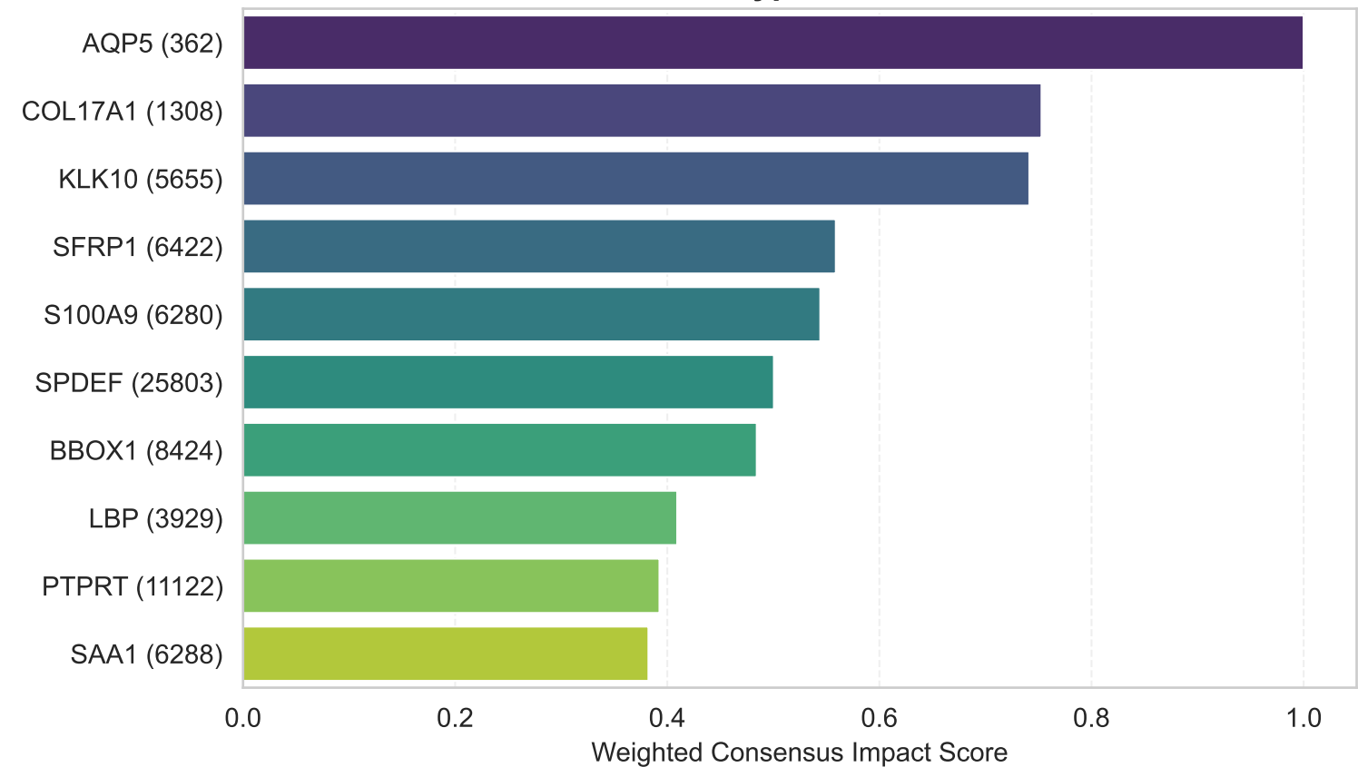
Subtype: LUMINAL_B
