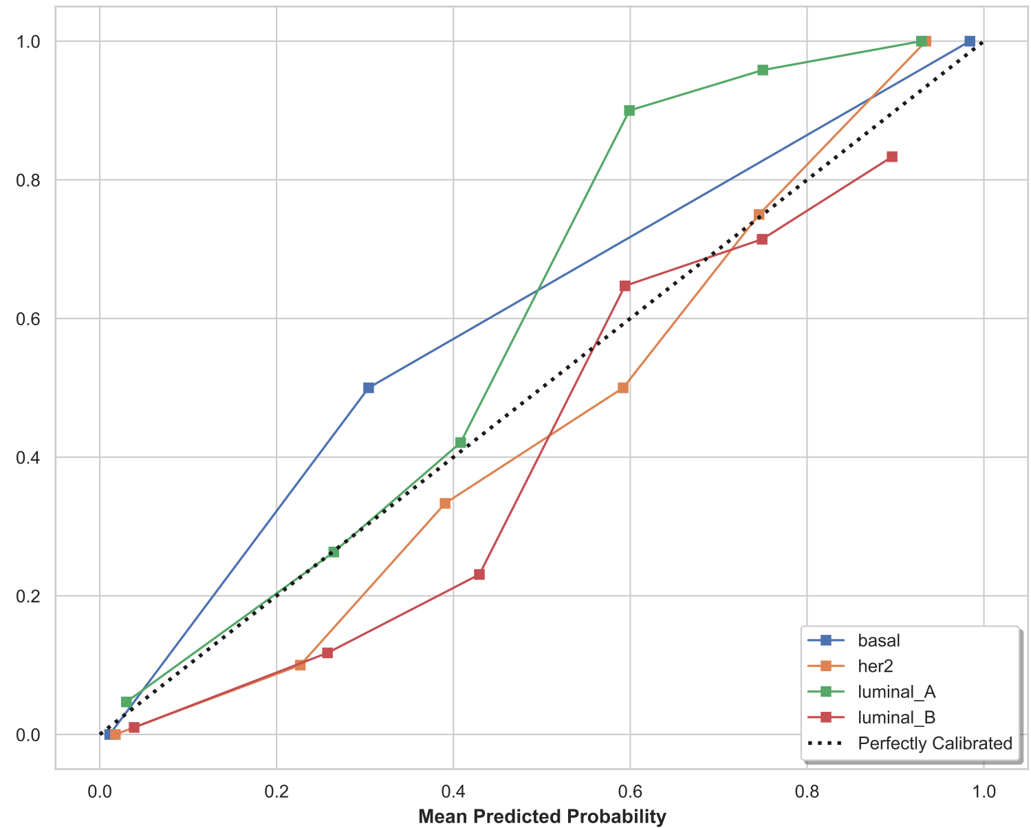
Logistic Regression (Linear) Proof of Probabilistic Reliability
