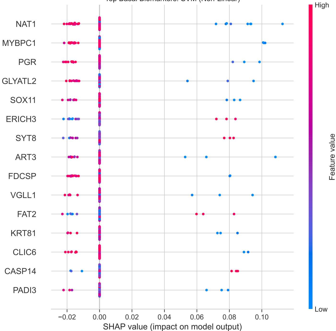
Top Basal Biomarkers: SVM (Non-Linear)
