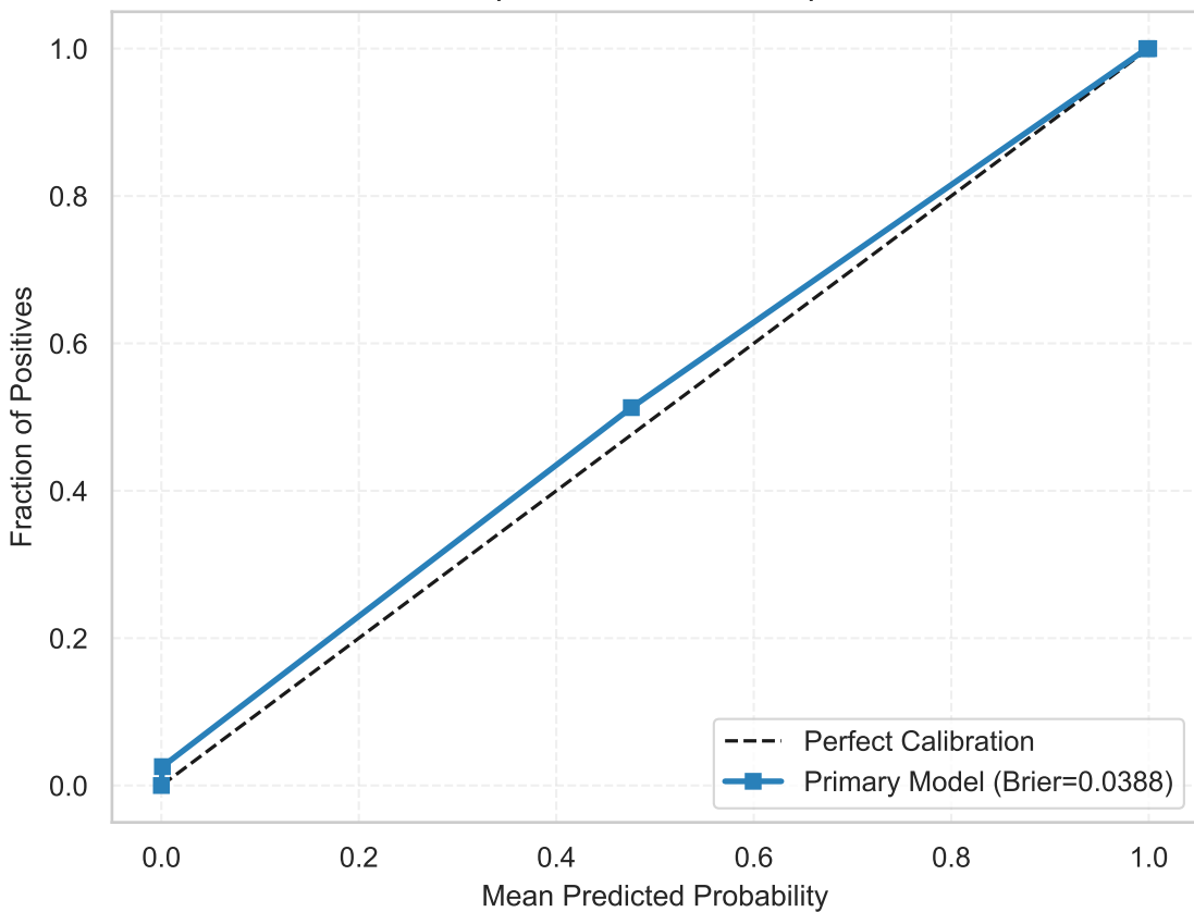
Clinical Reliability: Subtype LUMINAL_A (Brier Score = 0.0388)
