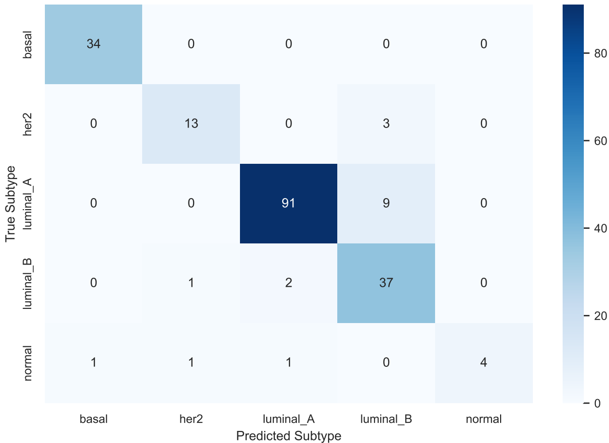
Confusion Matrix: RANDOM FOREST
