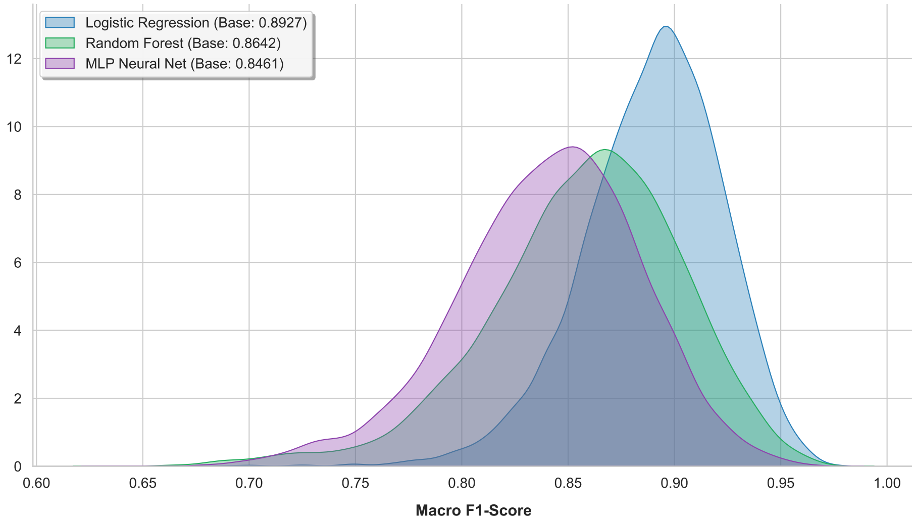
Bootstrap Distribution of Holdout Macro F1-Score (N=10,000)
