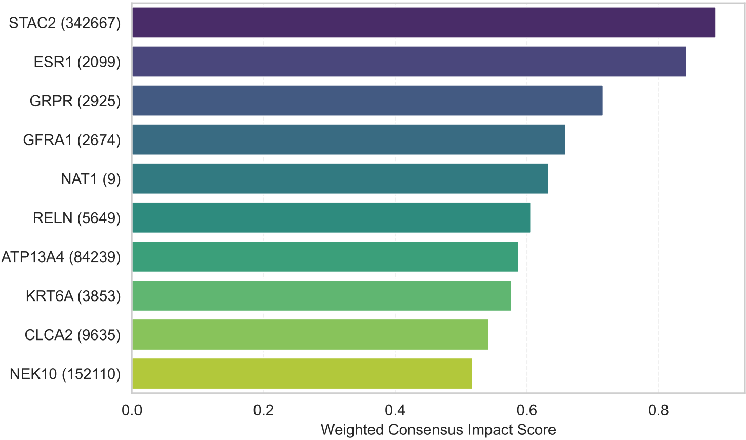
Subtype: NORMAL
