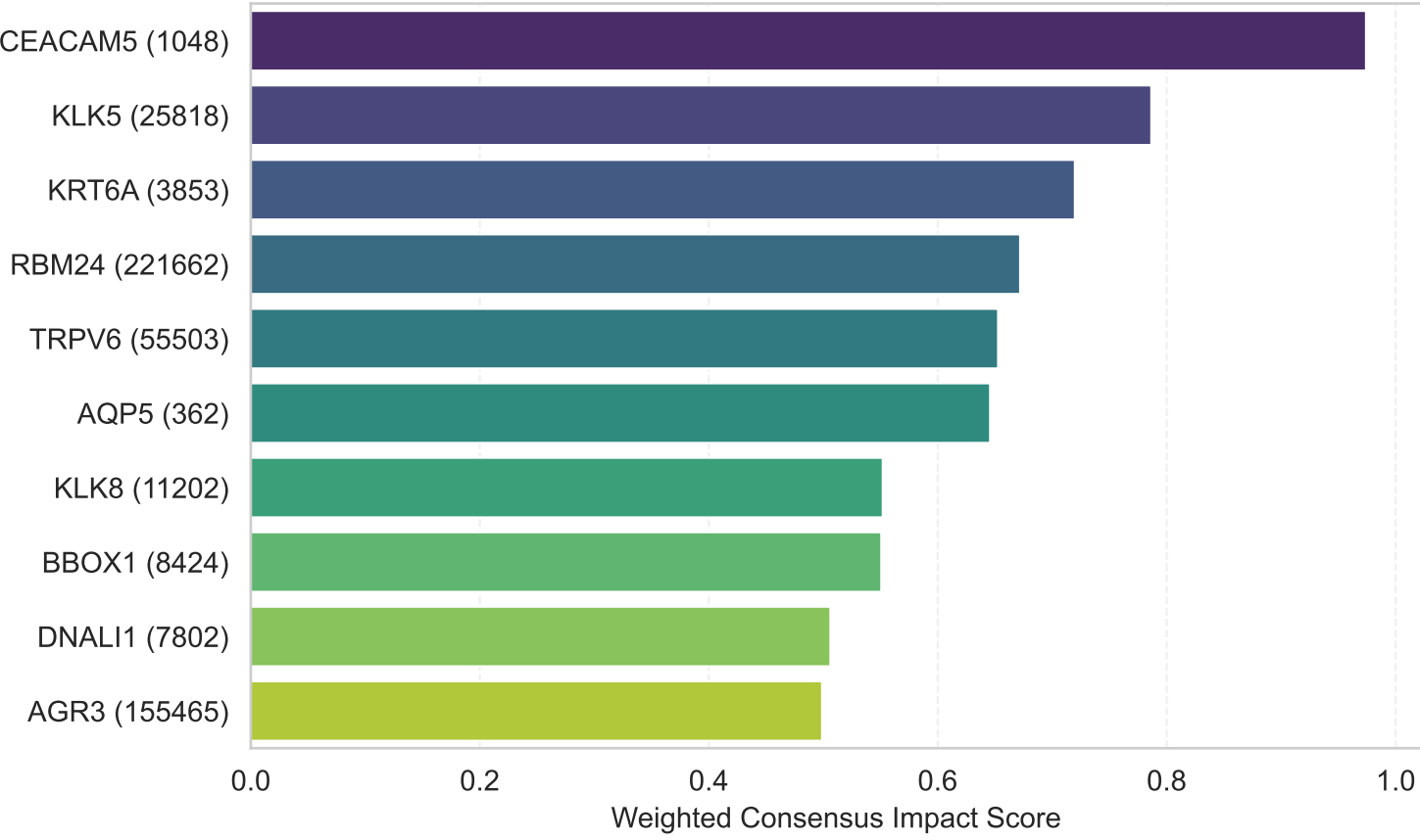
Subtype: LUMINAL_B
