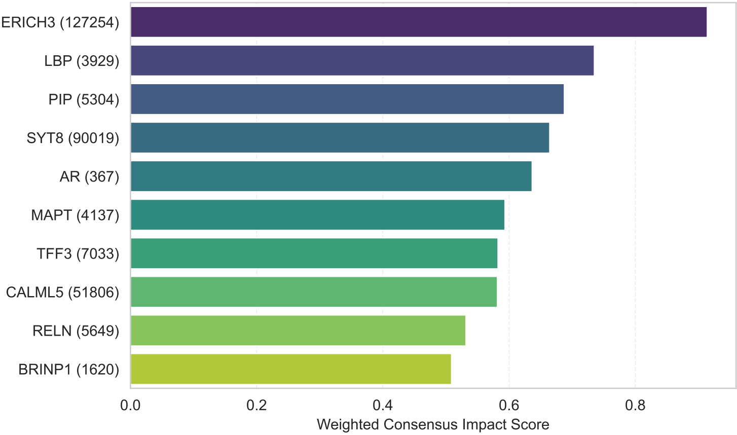
Subtype: LUMINAL_A
