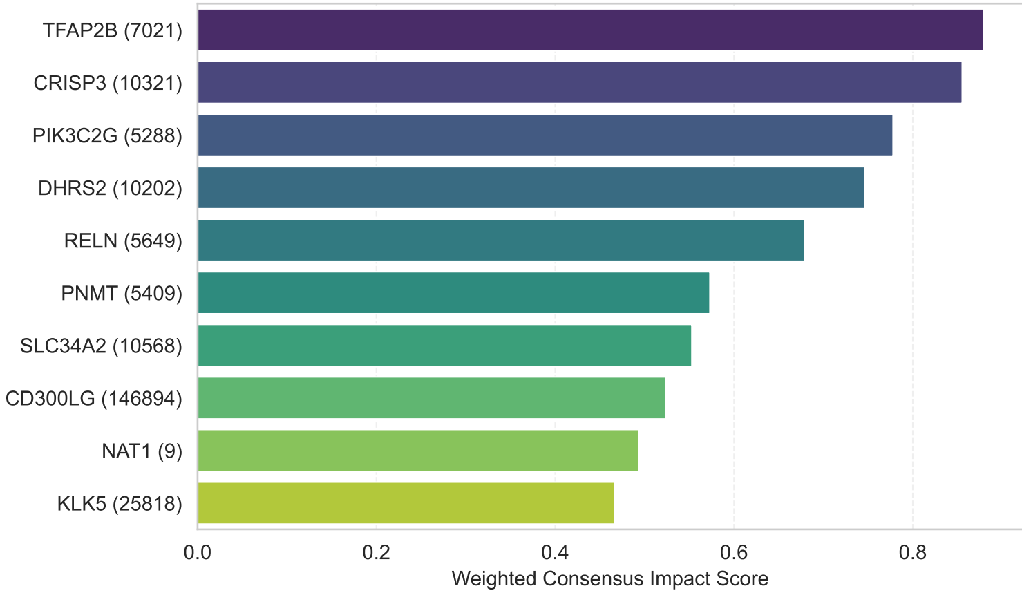
Subtype: LUMINAL_B
