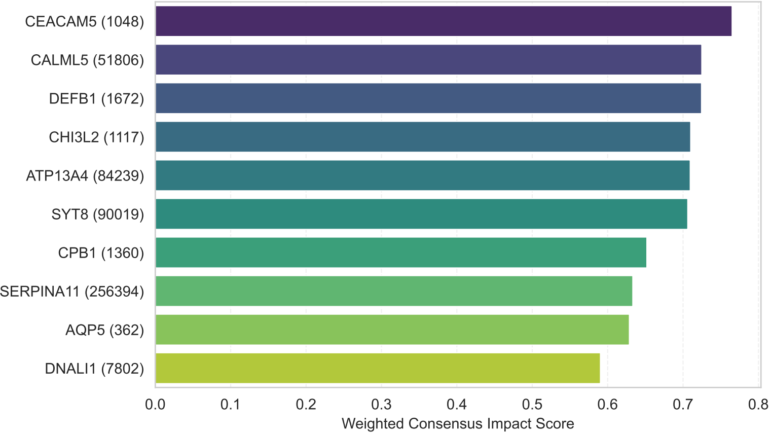
Subtype: NORMAL
